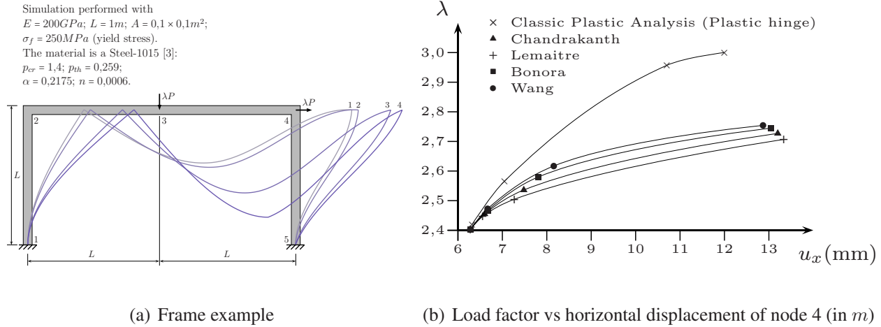
Fig. 3 Test on a 2D frame
