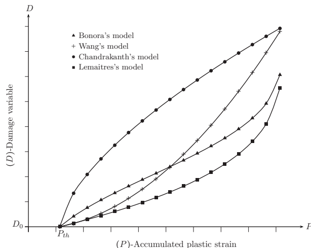
Fig. 2 Damage ( D ) versus accumulated plastic strain ( p )
